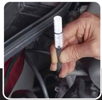
Flow meter quickly indicates presence of sealant
